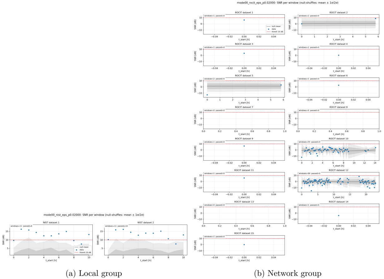
Figure 1: Mode n = 0 at \epsilon = 0.02 : SNR vs window start time. Null-shuffle bands ( \mu \pm \sigma and \mu \pm 2\sigma ) are shown. No windows are excluded.
