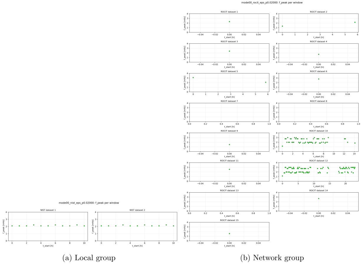
Figure 2: Mode n = 0 at \epsilon = 0.02 : f_{\text{peak}} vs window start time.
